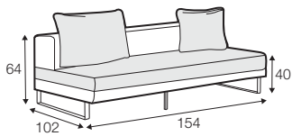
2,5 seater without armrests back cushion 54x54 and 72x54
