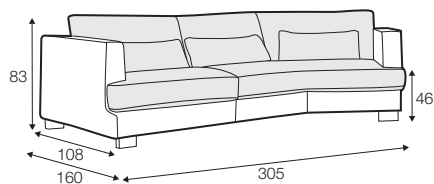
set 8 right / or left armchair left / or right + corner 35° right / or left
