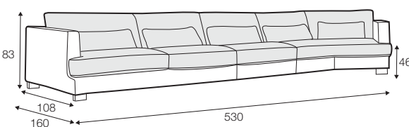
set 14 right / or left 3 seater left / or right + armchair wide without armrests + corner 35° right / or left
